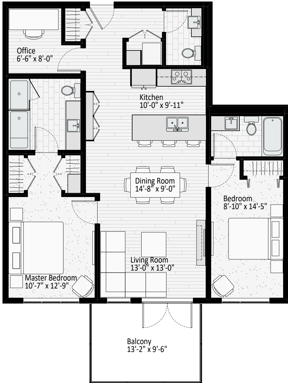
LEVEL 2 KEYPLAN
